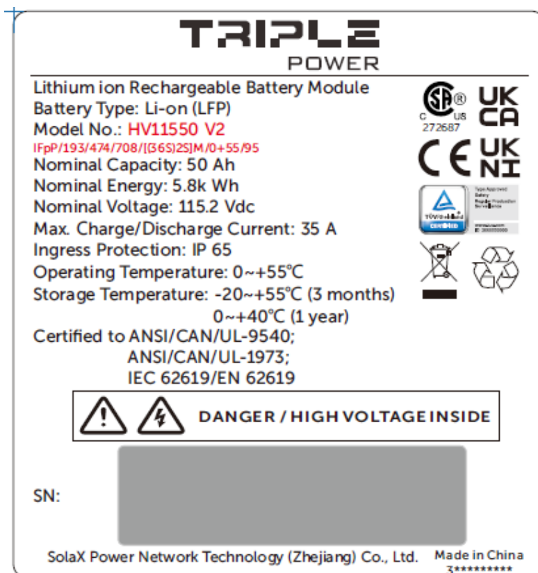
图 4 电池标签 Picture 4 Label of Battery
